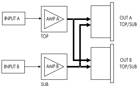
Input/Output routing "Mix TOP/SUB"*
